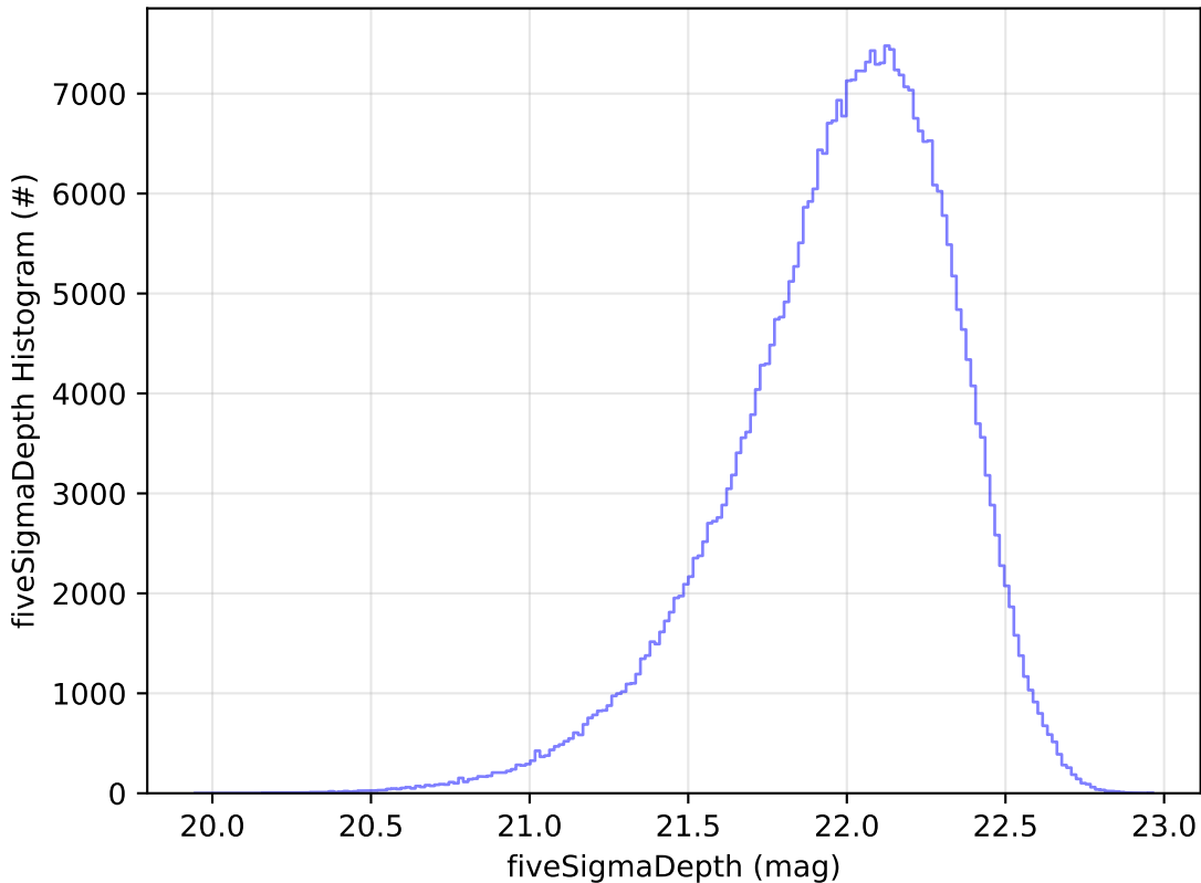
roll_uniform_eh_acc0.2_mjdp0_v3.4_10yrs y: fiveSigmaDepth Histogram
