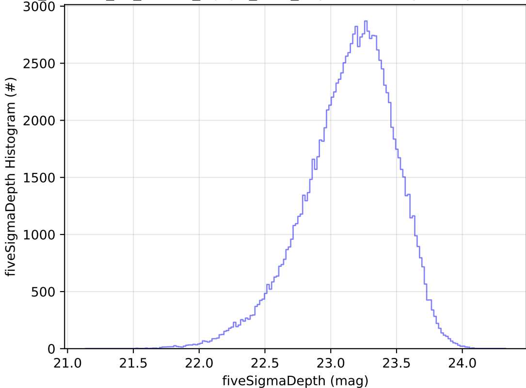
roll_uniform_eh_acc0.2_mjdp0_v3.4_10yrs u: fiveSigmaDepth Histogram
