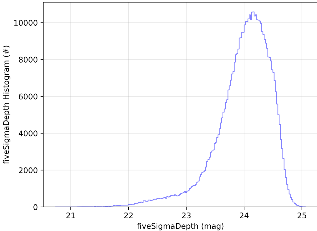
roll_uniform_eh_acc0.2_mjdp0_v3.4_10yrs r: fiveSigmaDepth Histogram
