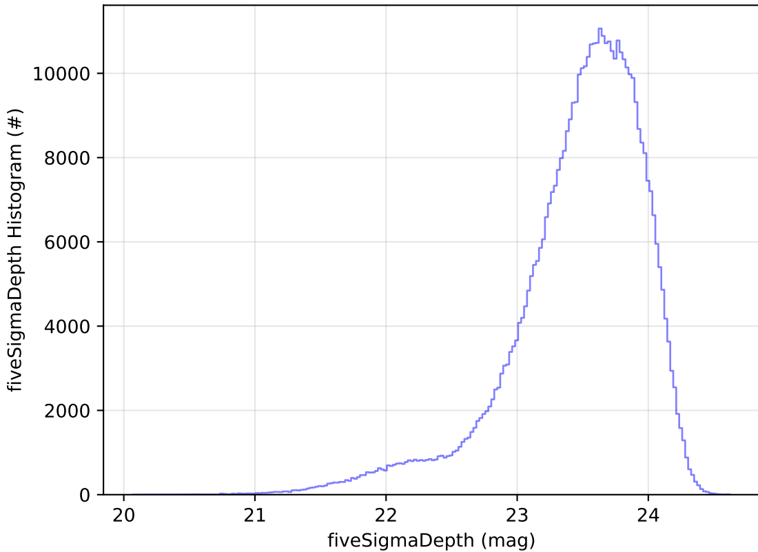
roll_uniform_eh_acc0.2_mjdp0_v3.4_10yrs i: fiveSigmaDepth Histogram
