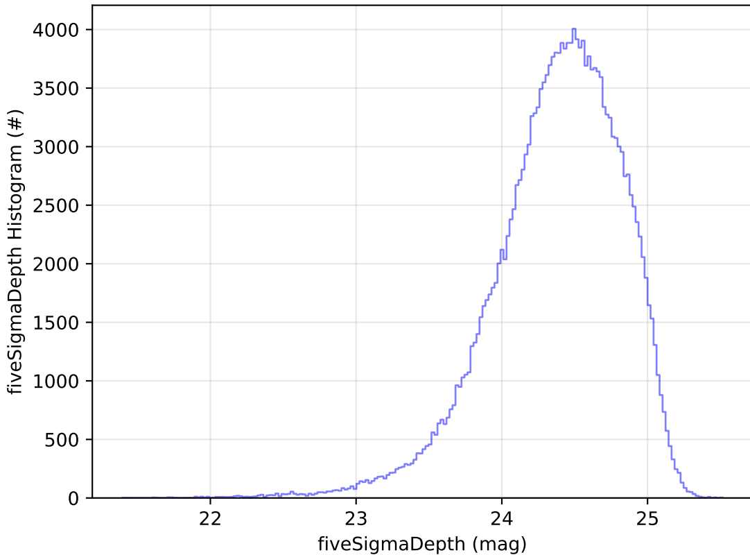
roll_uniform_eh_acc0.2_mjdp0_v3.4_10yrs g: fiveSigmaDepth Histogram
