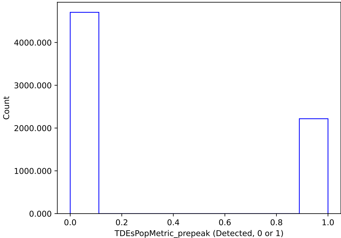
roll_uniform_eh_acc0.2_mjdp0_v3.4_10yrs : TDEsPopMetric_prepeak
