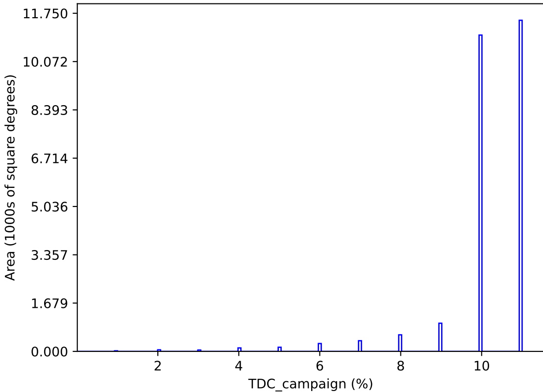
roll_uniform_eh_acc0.2_mjdp0_v3.4_10yrs : TDC_campaign
