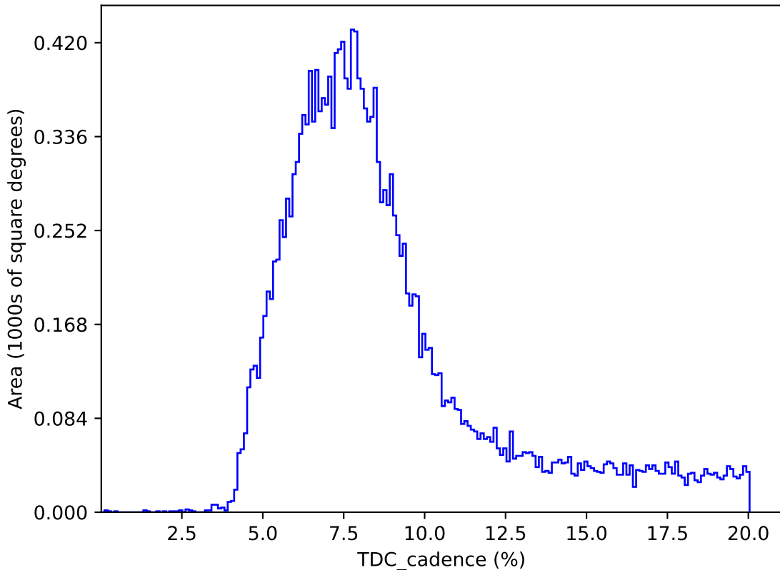
roll_uniform_eh_acc0.2_mjdp0_v3.4_10yrs : TDC_cadence
