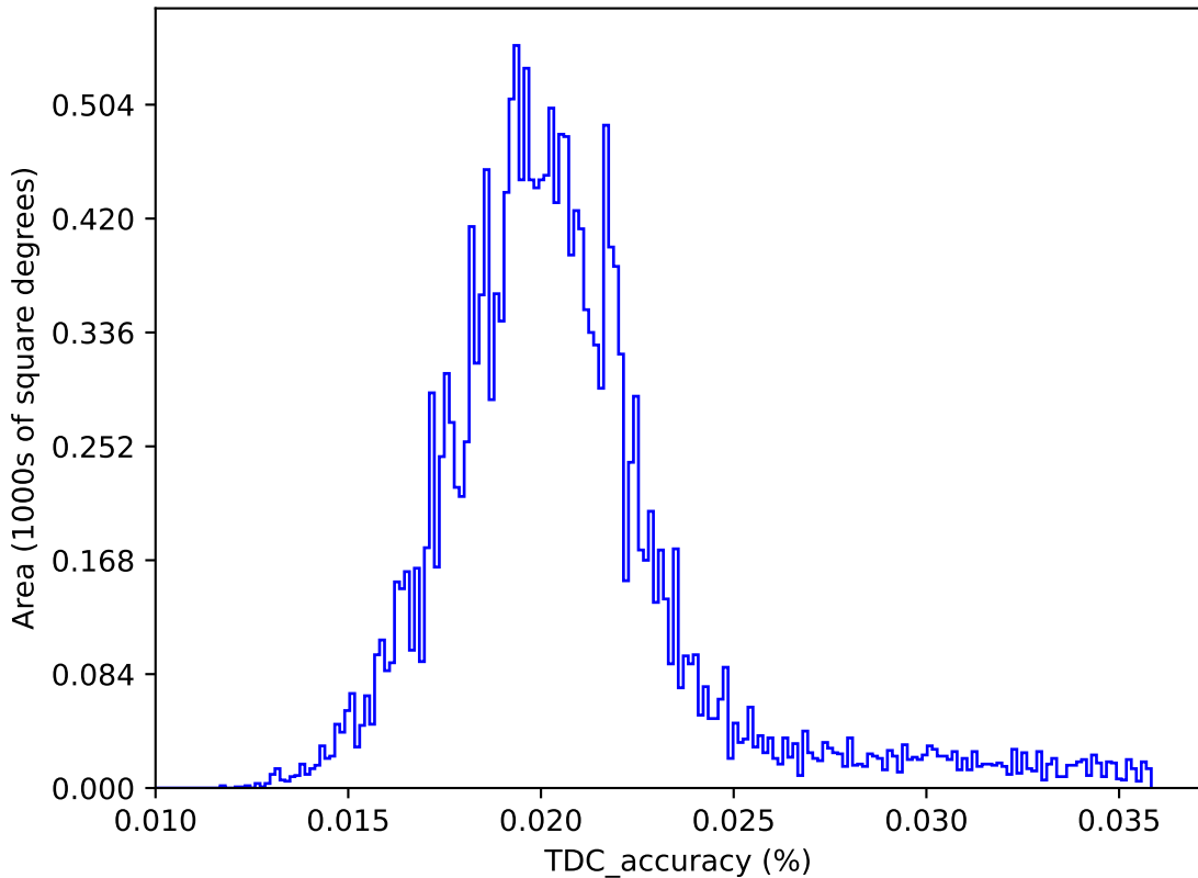
roll_uniform_eh_acc0.2_mjdp0_v3.4_10yrs : TDC_accuracy
