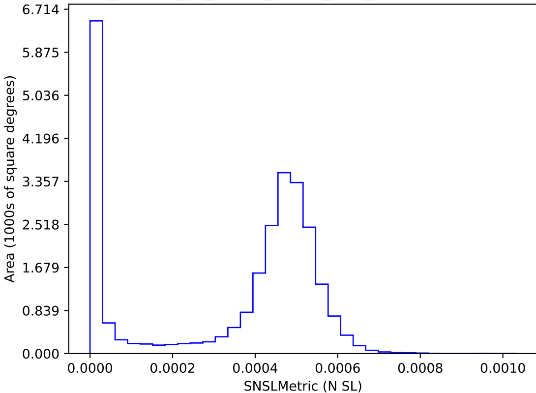
roll_uniform_eh_acc0.2_mjdp0_v3.4_10yrs : SNSLMetric
