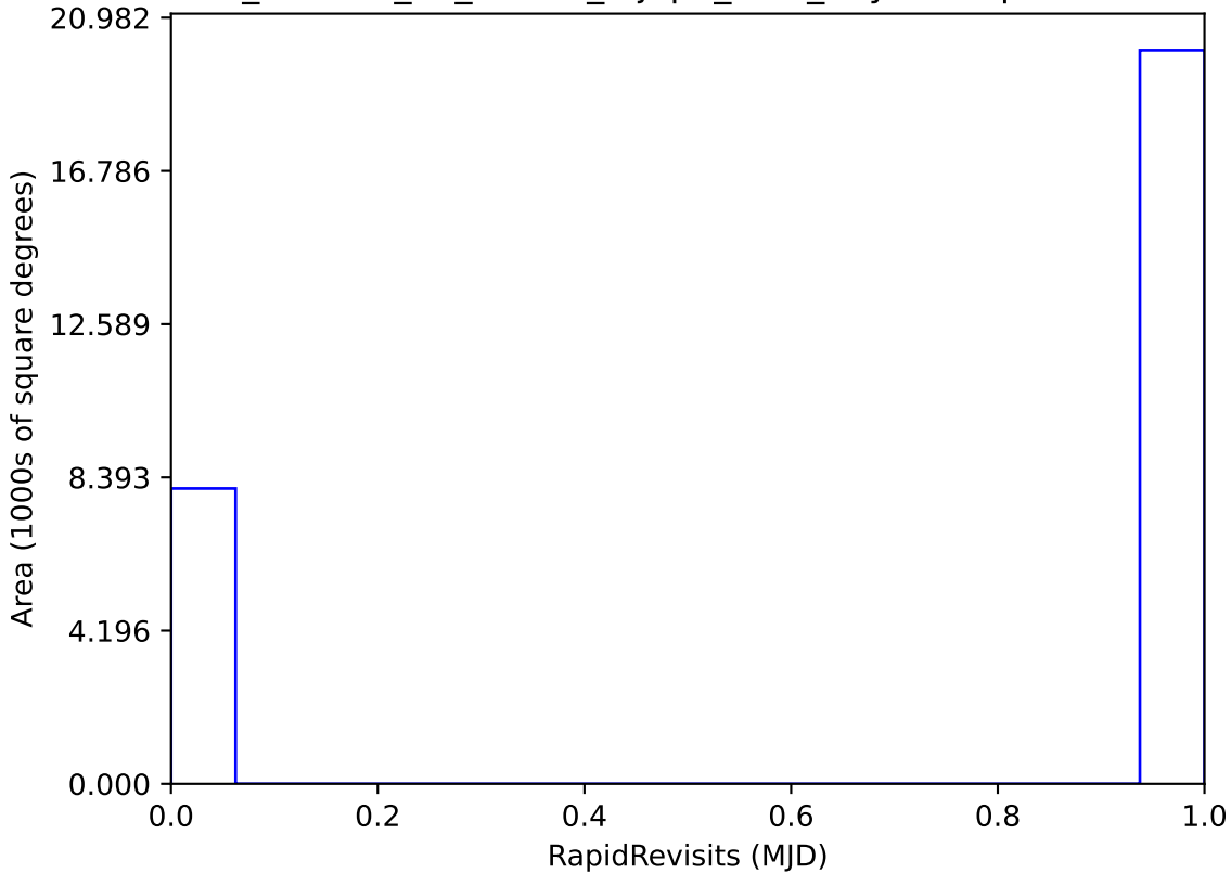
roll_uniform_eh_acc0.2_mjdp0_v3.4_10yrs : RapidRevisits
