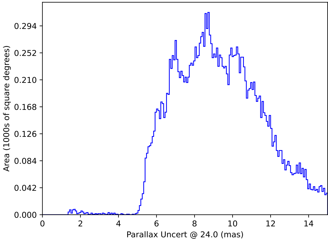
roll_uniform_eh_acc0.2_mjdp0_v3.4_10yrs : Parallax Uncert @ 24.0
