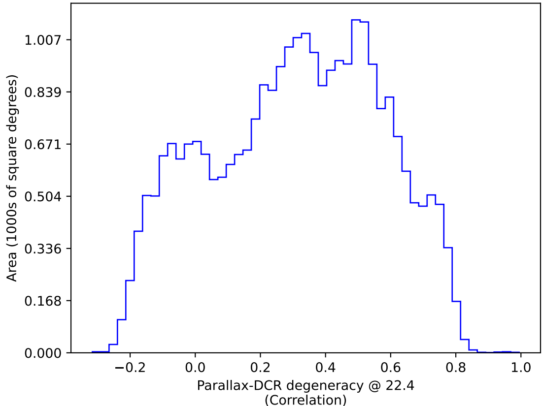
roll_uniform_eh_acc0.2_mjdp0_v3.4_10yrs : Parallax-DCR degeneracy @ 22.4
