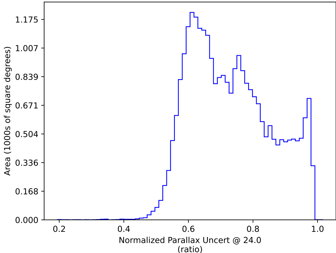
roll_uniform_eh_acc0.2_mjdp0_v3.4_10yrs : Normalized Parallax Uncert @ 24.0
