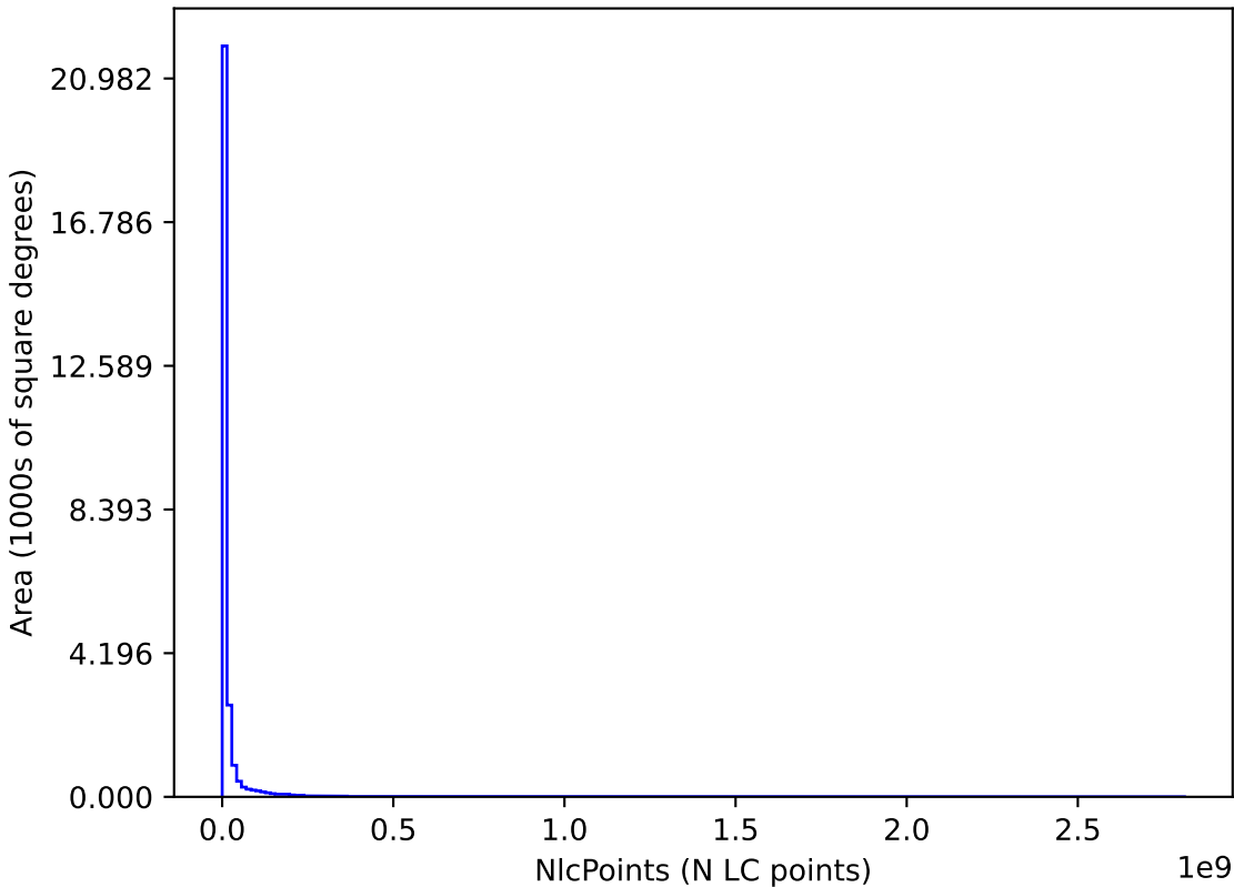
roll_uniform_eh_acc0.2_mjdp0_v3.4_10yrs : NlcPoints
