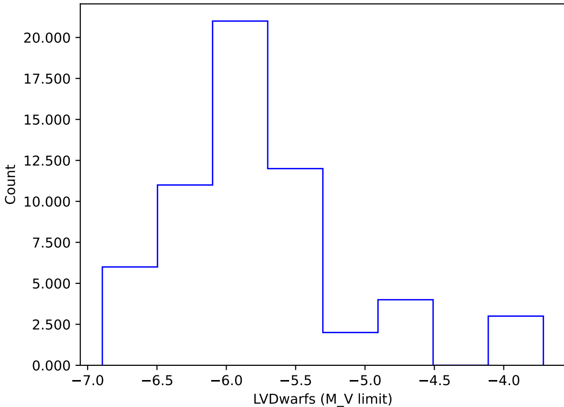
roll_uniform_eh_acc0.2_mjdp0_v3.4_10yrs gi: LVDwarfs
