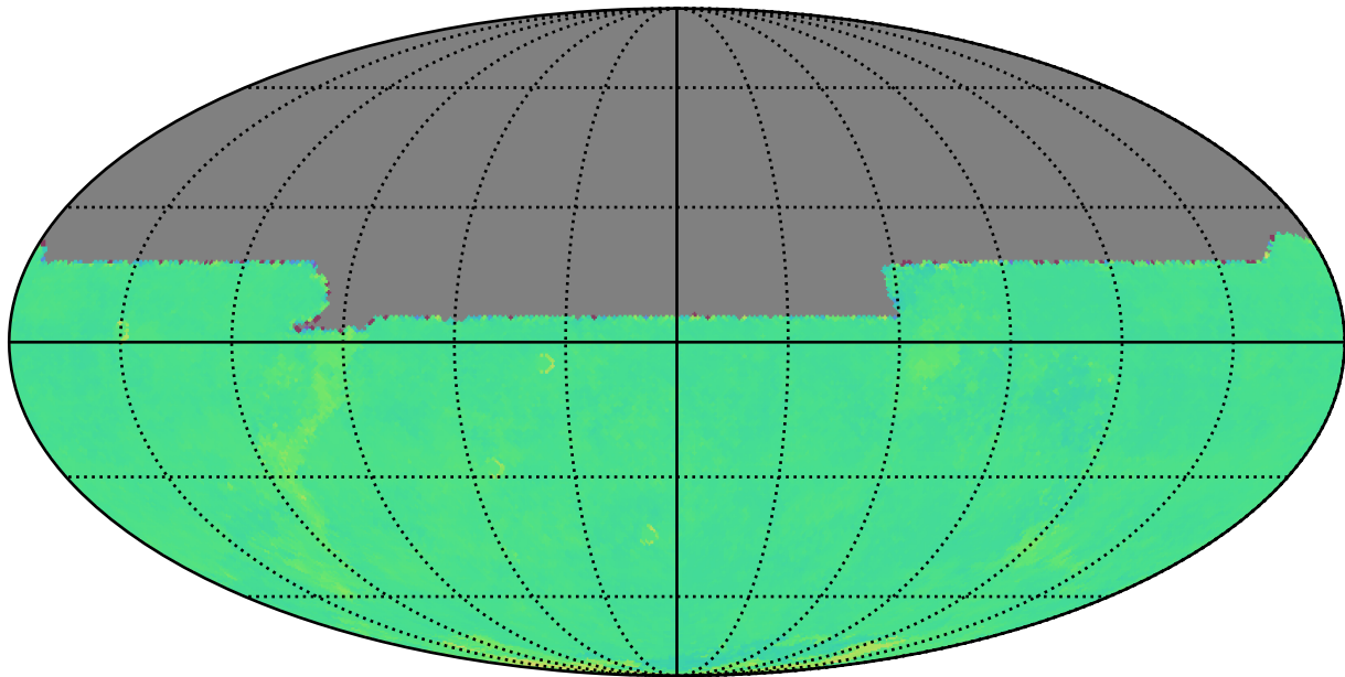
roll_uniform_eh_acc0.2_mjdp0_v3.4_10yrs y: Kuiper rotTelPos
