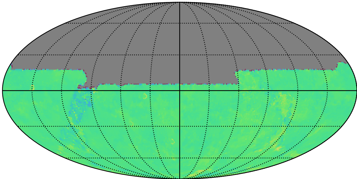
roll_uniform_eh_acc0.2_mjdp0_v3.4_10yrs u: Kuiper rotTelPos
