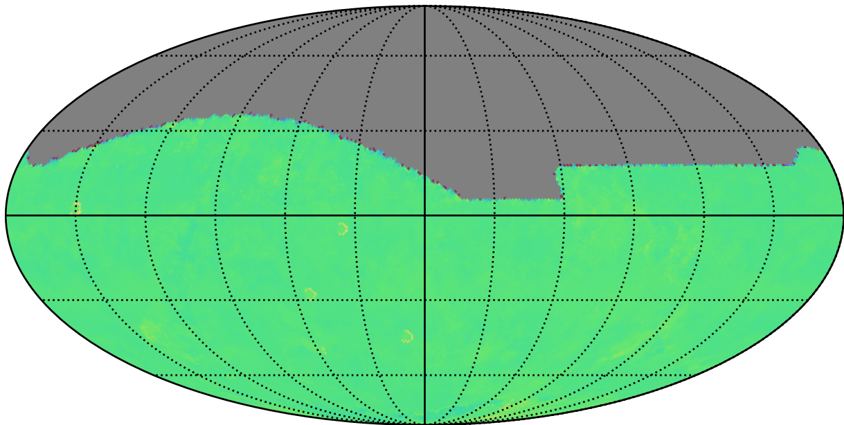
roll_uniform_eh_acc0.2_mjdp0_v3.4_10yrs r: Kuiper rotTelPos
