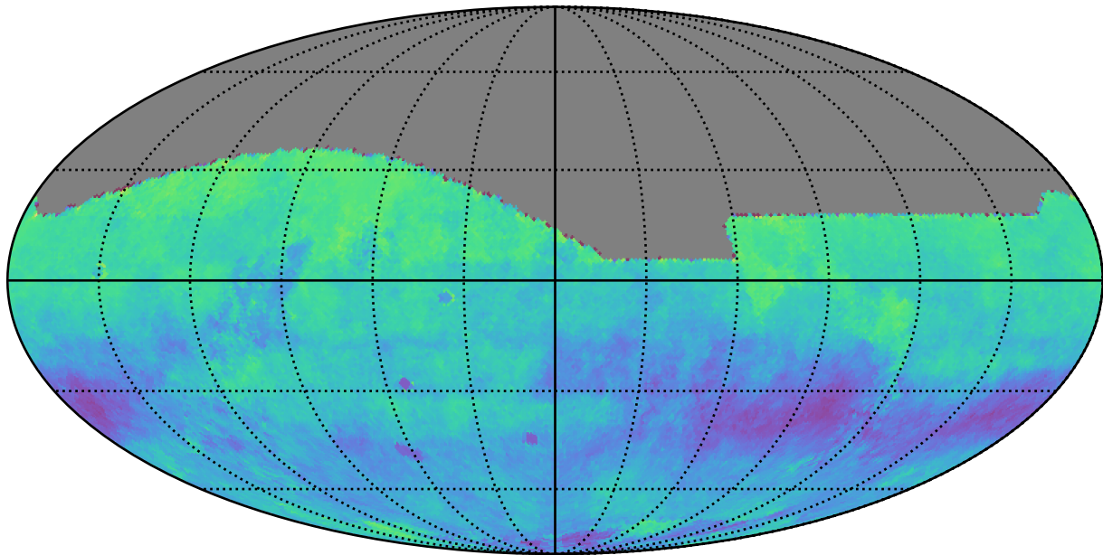
roll_uniform_eh_acc0.2_mjdp0_v3.4_10yrs r: Kuiper rotSkyPos
