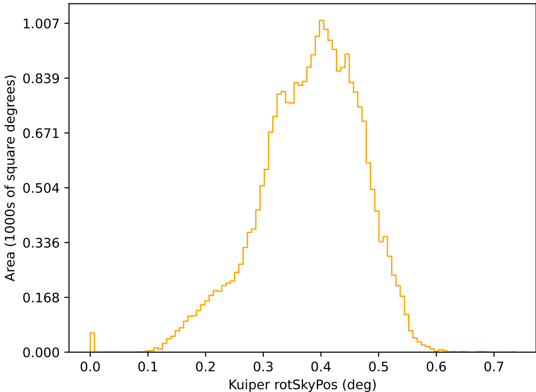
roll_uniform_eh_acc0.2_mjdp0_v3.4_10yrs r: Kuiper rotSkyPos
