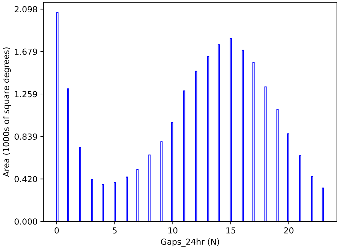
roll_uniform_eh_acc0.2_mjdp0_v3.4_10yrs y band: Gaps_24hr
