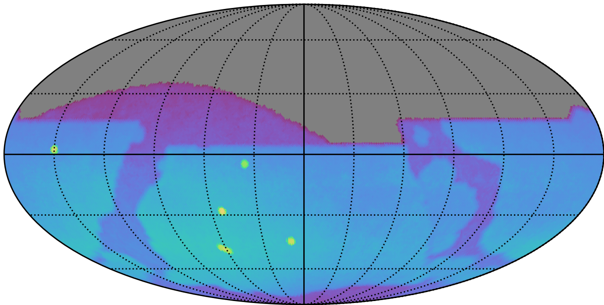
roll_uniform_eh_acc0.2_mjdp0_v3.4_10yrs : Brown Dwarf, L7
