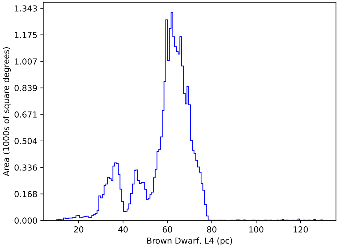
roll_uniform_eh_acc0.2_mjdp0_v3.4_10yrs : Brown Dwarf, L4
