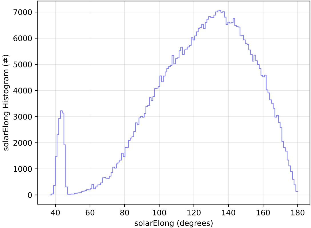
roll_uniform_eh_acc0.2_mjdp0_v3.4_10yrs WFD r band: solarElong Histogram
