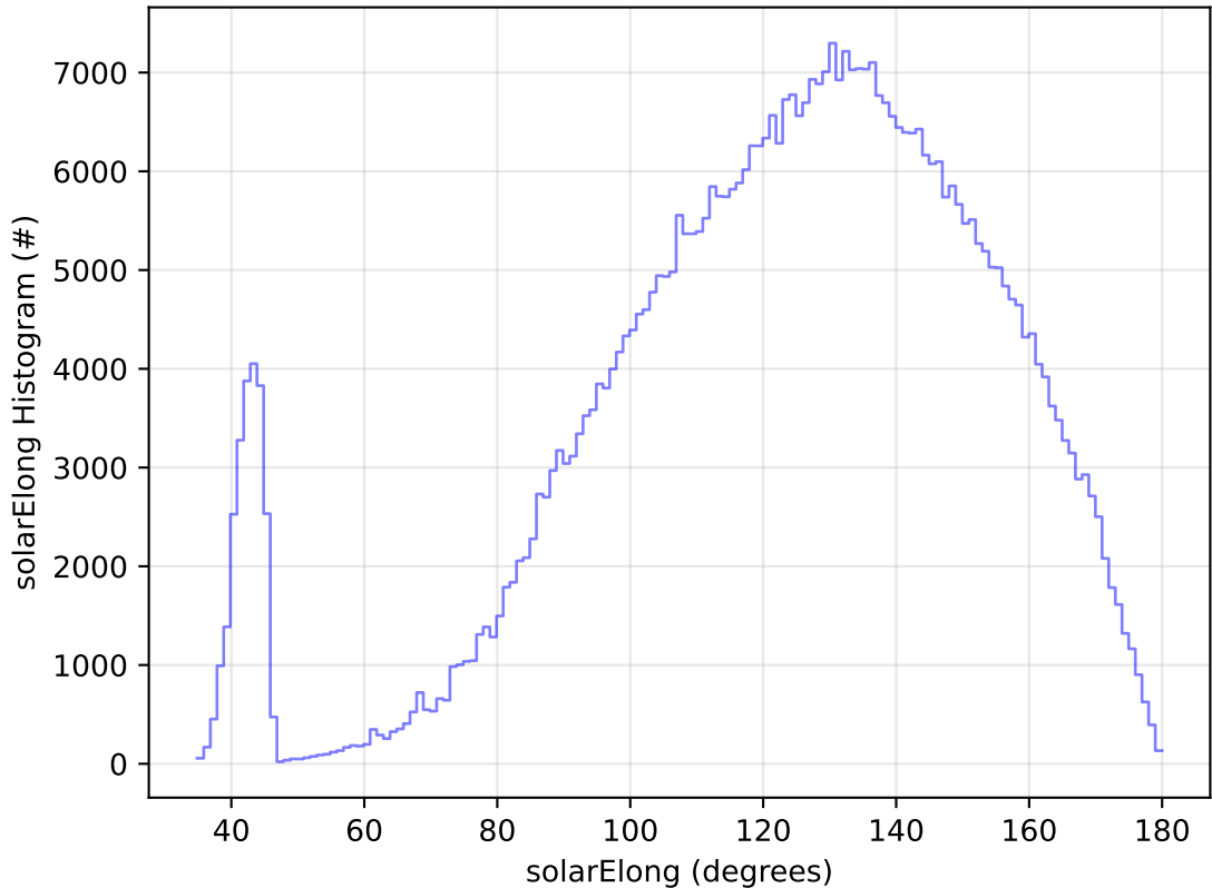
roll_uniform_eh_acc0.2_mjdp0_v3.4_10yrs WFD i band: solarElong Histogram
