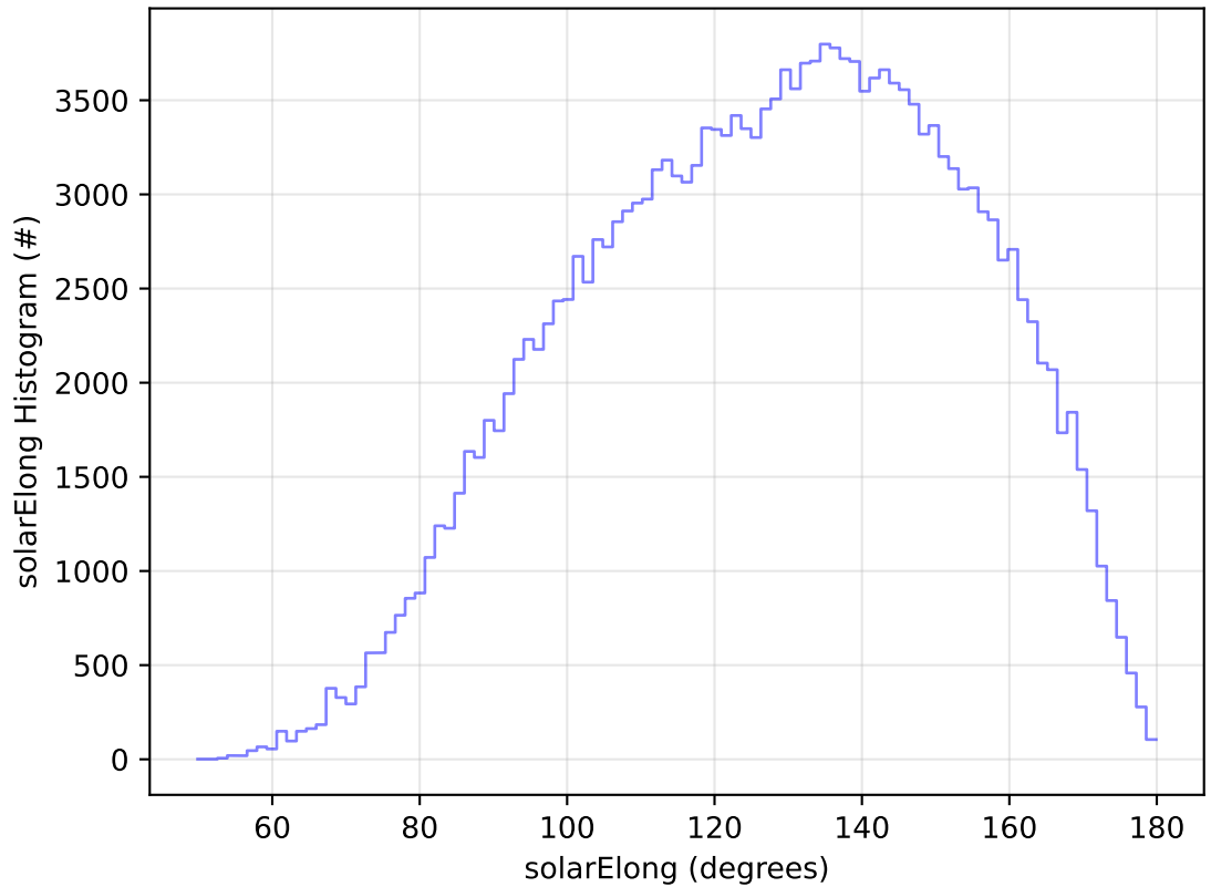
roll_uniform_eh_acc0.2_mjdp0_v3.4_10yrs WFD g band: solarElong Histogram
