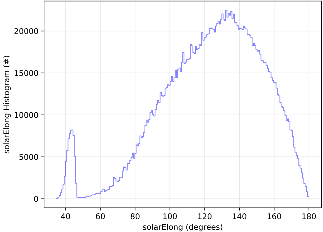
roll_uniform_eh_acc0.2_mjdp0_v3.4_10yrs WFD all bands: solarElong Histogram
