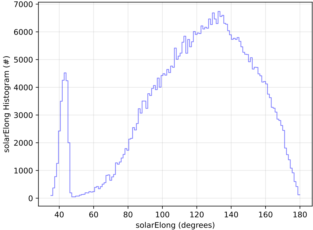
roll_uniform_eh_acc0.2_mjdp0_v3.4_10yrs All sky z band: solarElong Histogram
