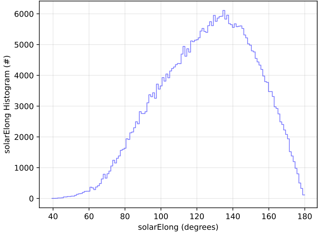
roll_uniform_eh_acc0.2_mjdp0_v3.4_10yrs All sky y band: solarElong Histogram
