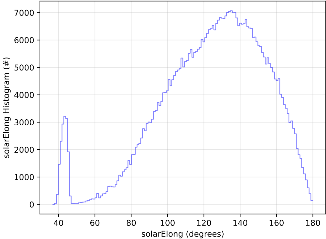
roll_uniform_eh_acc0.2_mjdp0_v3.4_10yrs All sky r band: solarElong Histogram
