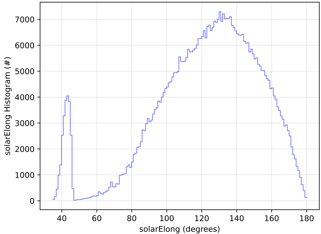
roll_uniform_eh_acc0.2_mjdp0_v3.4_10yrs All sky i band: solarElong Histogram
