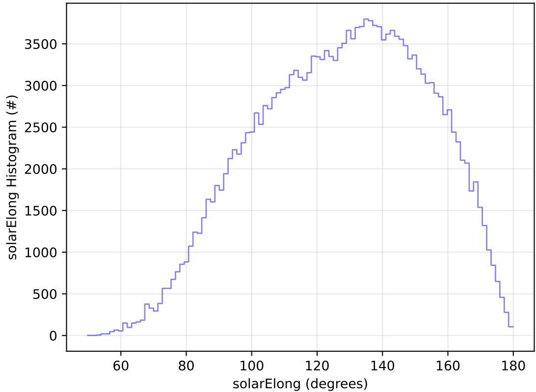
roll_uniform_eh_acc0.2_mjdp0_v3.4_10yrs All sky g band: solarElong Histogram
