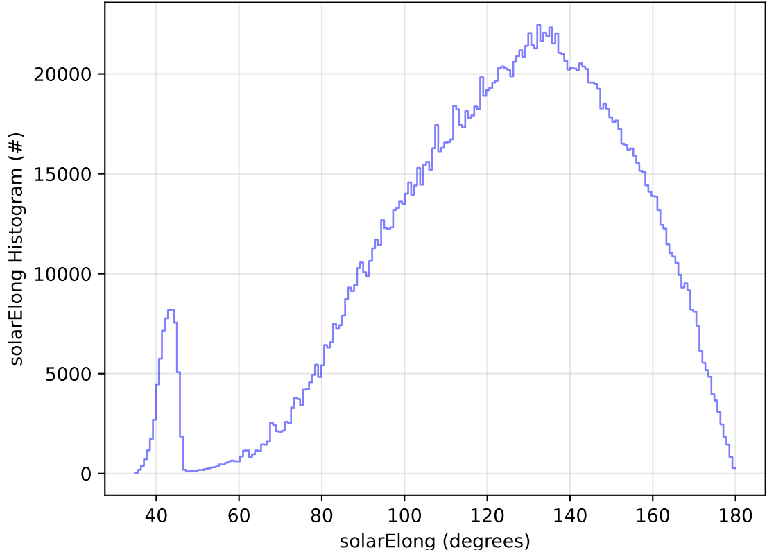
roll_uniform_eh_acc0.2_mjdp0_v3.4_10yrs All sky all bands: solarElong Histogram
