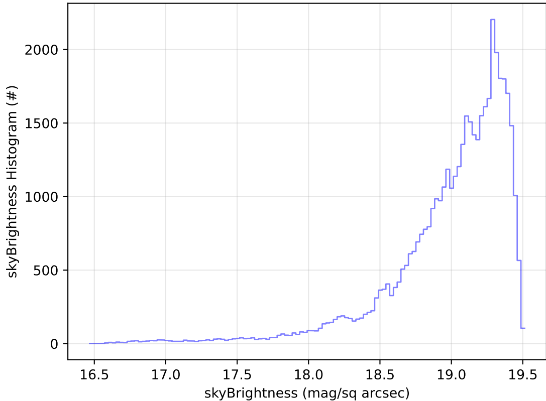
roll_uniform_eh_acc0.2_mjdp0_v3.4_10yrs Yr 1 z band: skyBrightness Histogram
