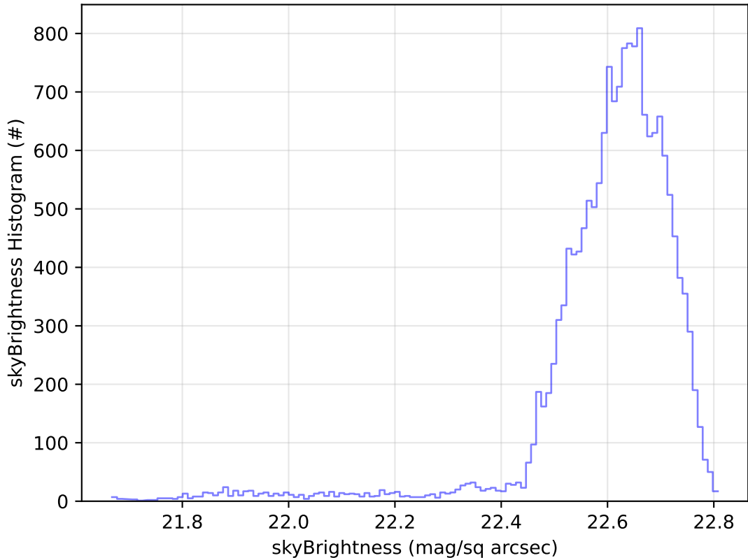
roll_uniform_eh_acc0.2_mjdp0_v3.4_10yrs Yr 1 u band: skyBrightness Histogram
