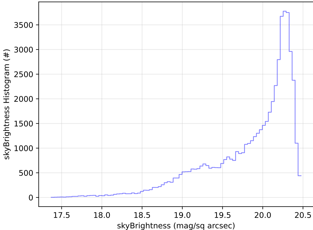
roll_uniform_eh_acc0.2_mjdp0_v3.4_10yrs Yr 1 i band: skyBrightness Histogram
