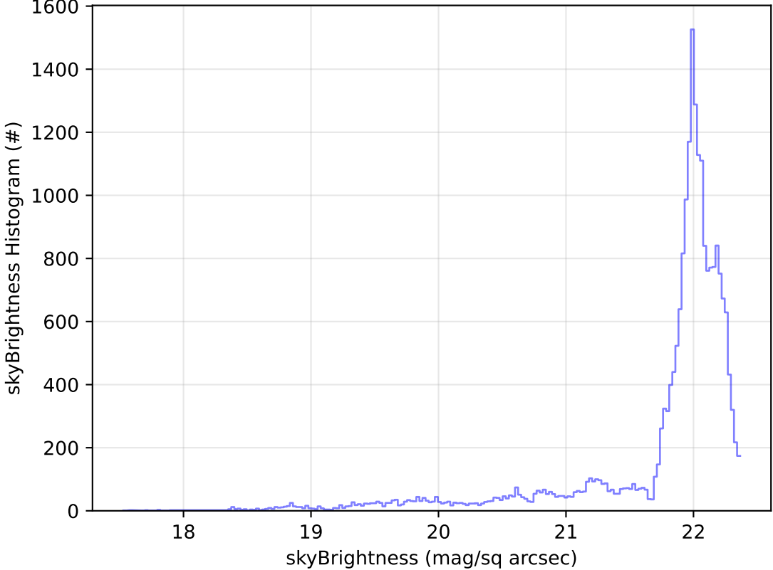
roll_uniform_eh_acc0.2_mjdp0_v3.4_10yrs Yr 1 g band: skyBrightness Histogram
