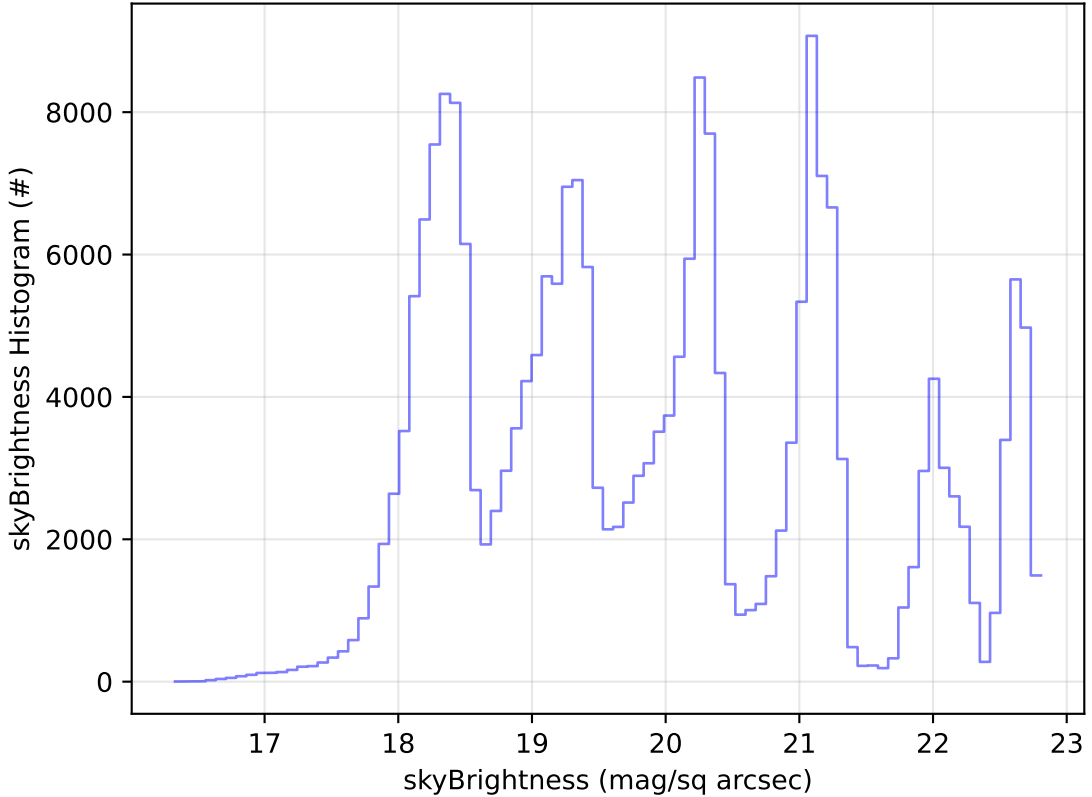
roll_uniform_eh_acc0.2_mjdp0_v3.4_10yrs Yr 1 all bands: skyBrightness Histogram
