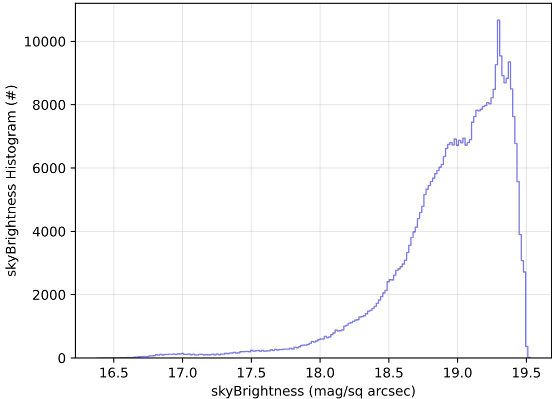
roll_uniform_eh_acc0.2_mjdp0_v3.4_10yrs WFD z band: skyBrightness Histogram
