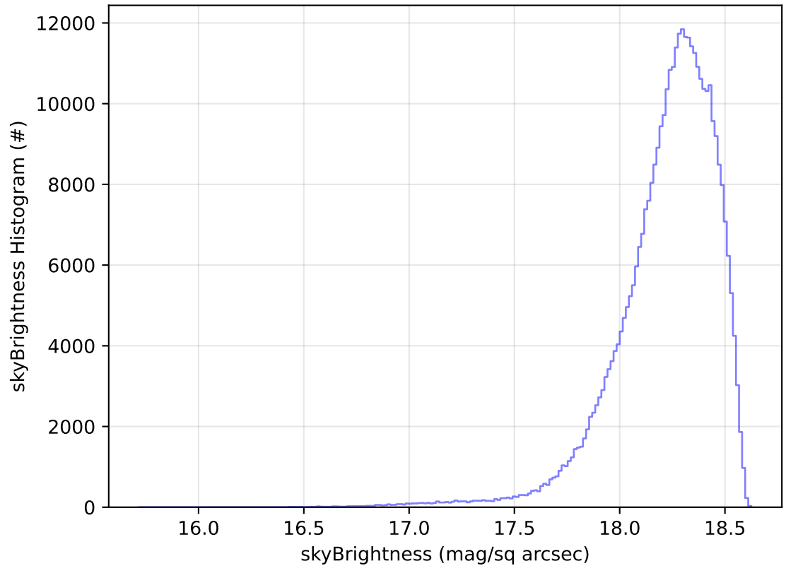
roll_uniform_eh_acc0.2_mjdp0_v3.4_10yrs WFD y band: skyBrightness Histogram
