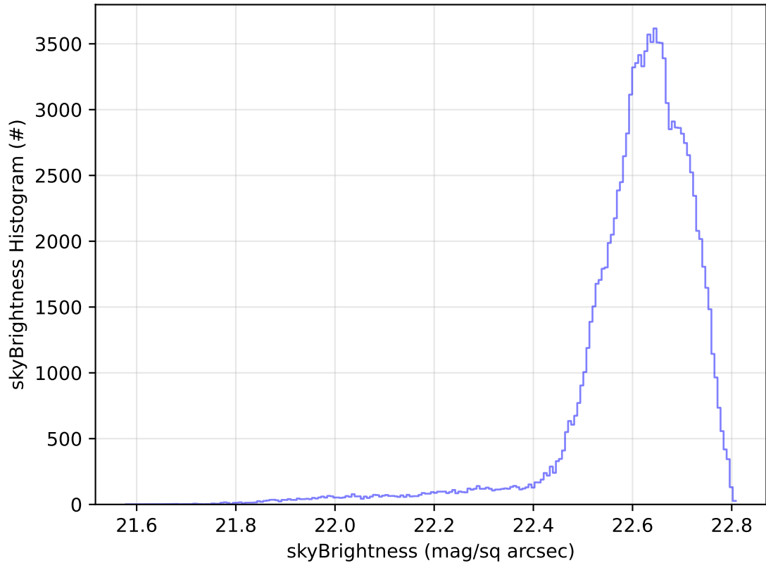
roll_uniform_eh_acc0.2_mjdp0_v3.4_10yrs WFD u band: skyBrightness Histogram
