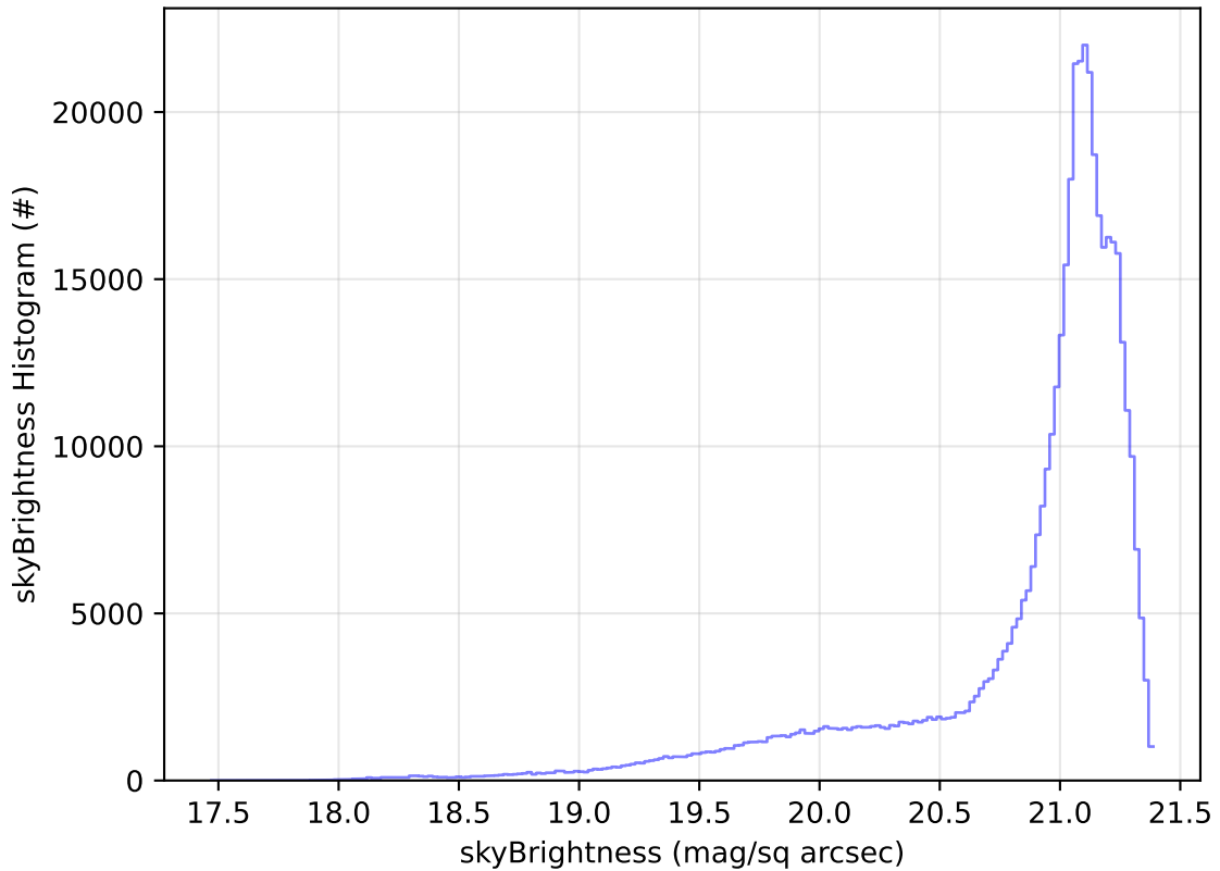
roll_uniform_eh_acc0.2_mjdp0_v3.4_10yrs WFD r band: skyBrightness Histogram
