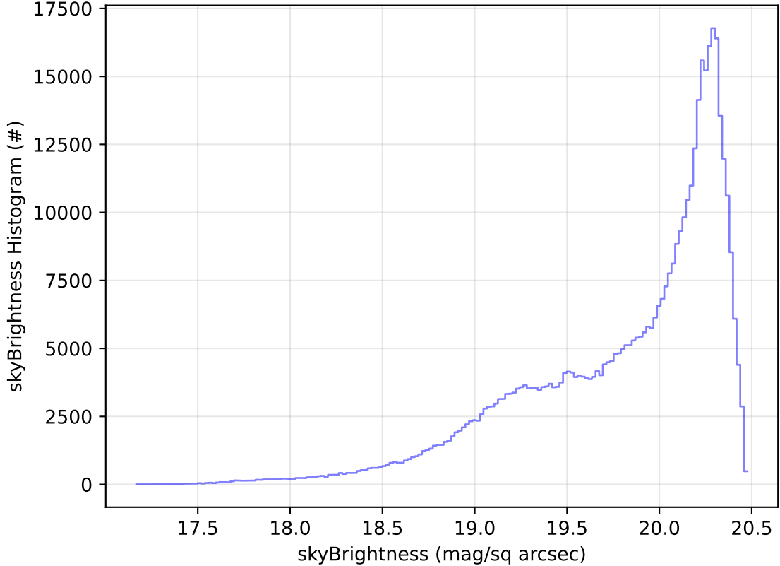
roll_uniform_eh_acc0.2_mjdp0_v3.4_10yrs WFD i band: skyBrightness Histogram
