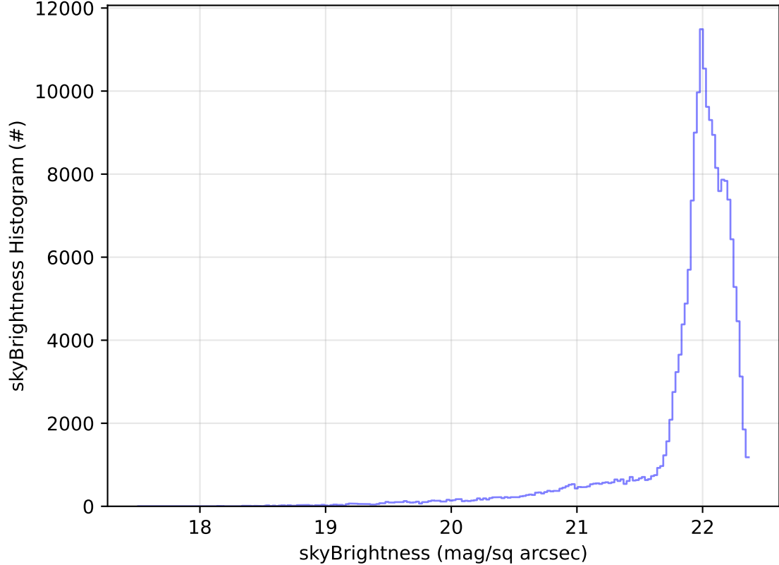
roll_uniform_eh_acc0.2_mjdp0_v3.4_10yrs WFD g band: skyBrightness Histogram
