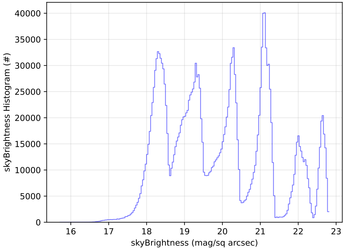
roll_uniform_eh_acc0.2_mjdp0_v3.4_10yrs WFD all bands: skyBrightness Histogram
