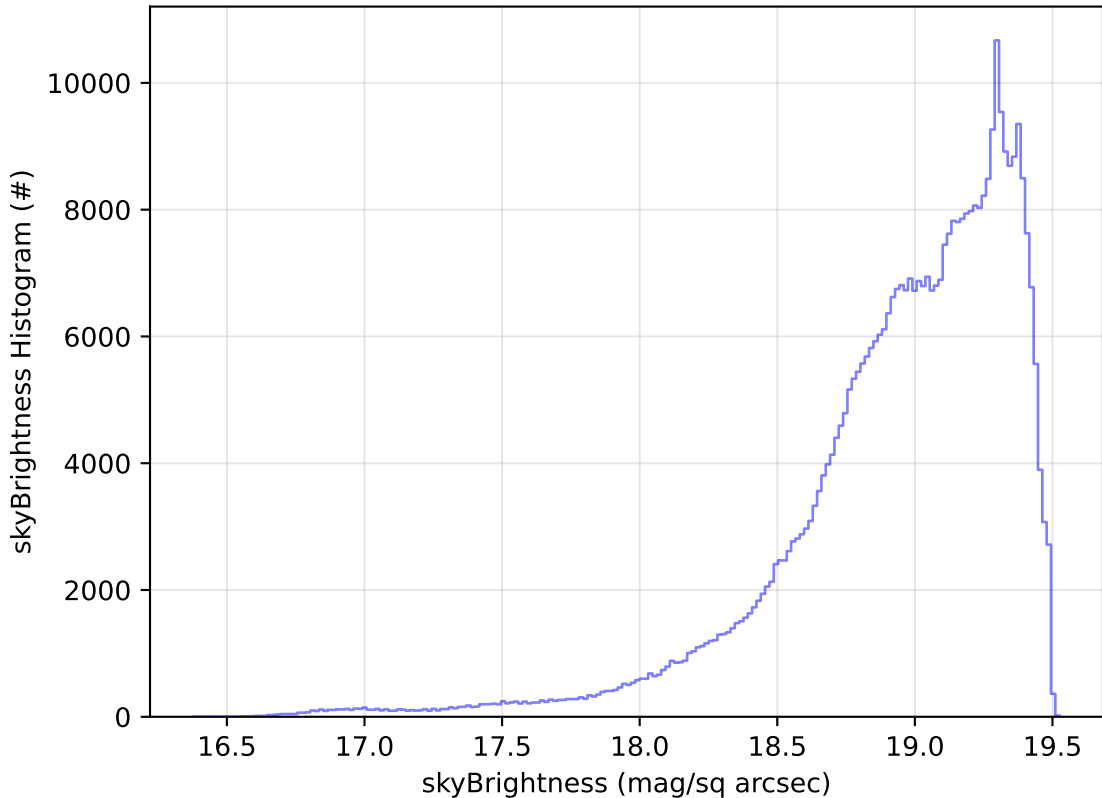
roll_uniform_eh_acc0.2_mjdp0_v3.4_10yrs All sky z band: skyBrightness Histogram
