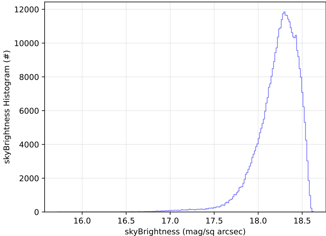
roll_uniform_eh_acc0.2_mjdp0_v3.4_10yrs All sky y band: skyBrightness Histogram
