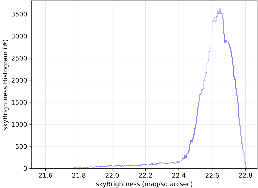
roll_uniform_eh_acc0.2_mjdp0_v3.4_10yrs All sky u band: skyBrightness Histogram
