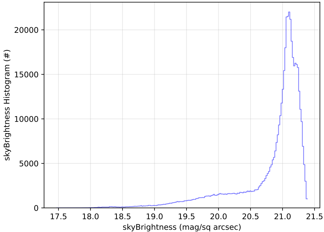
roll_uniform_eh_acc0.2_mjdp0_v3.4_10yrs All sky r band: skyBrightness Histogram
